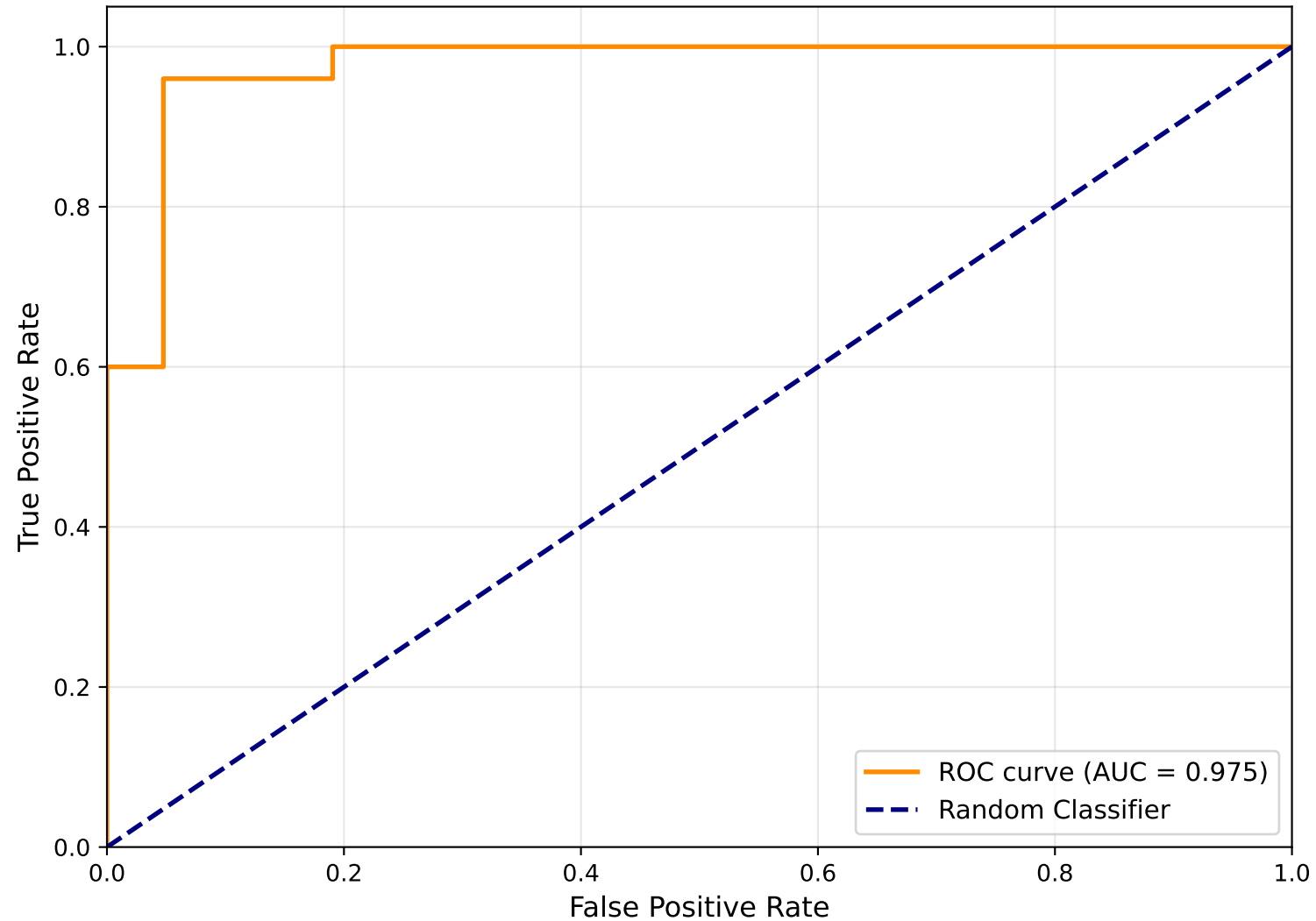
ROC Curve for Stacking Ensemble
